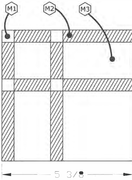
Zero grout line pattern (Butt Joint)
